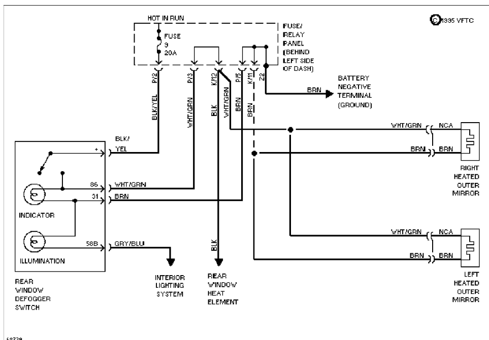
Heated Mirrors Circuit
