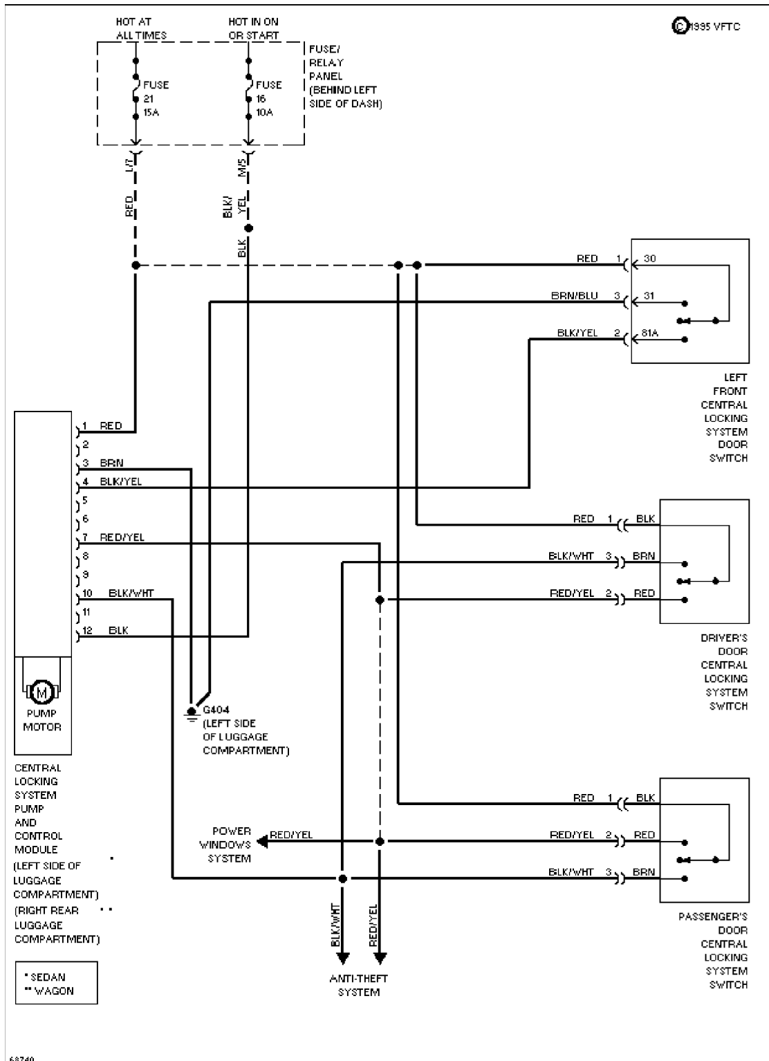
Power Door Lock Circuit
