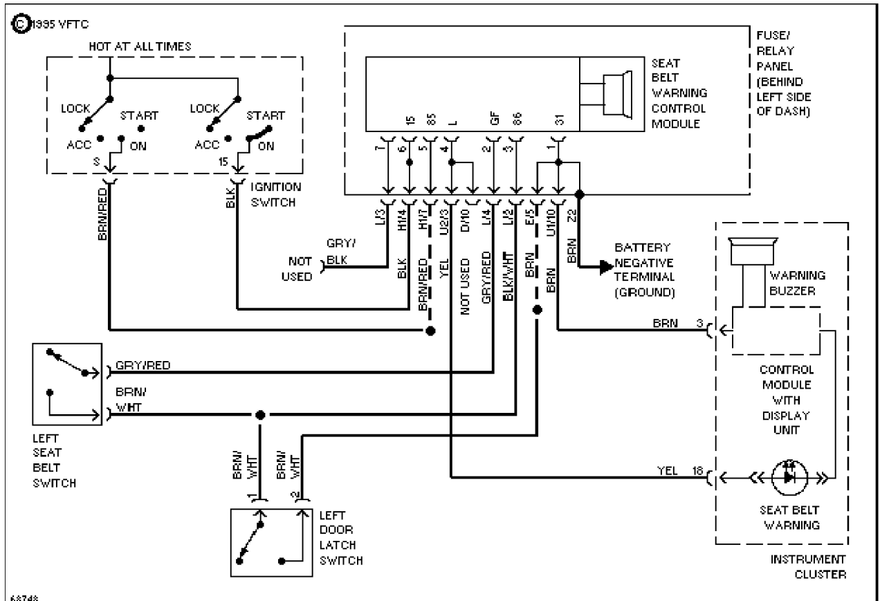
Warning System Circuits, W/O Automatic Seatbelts
