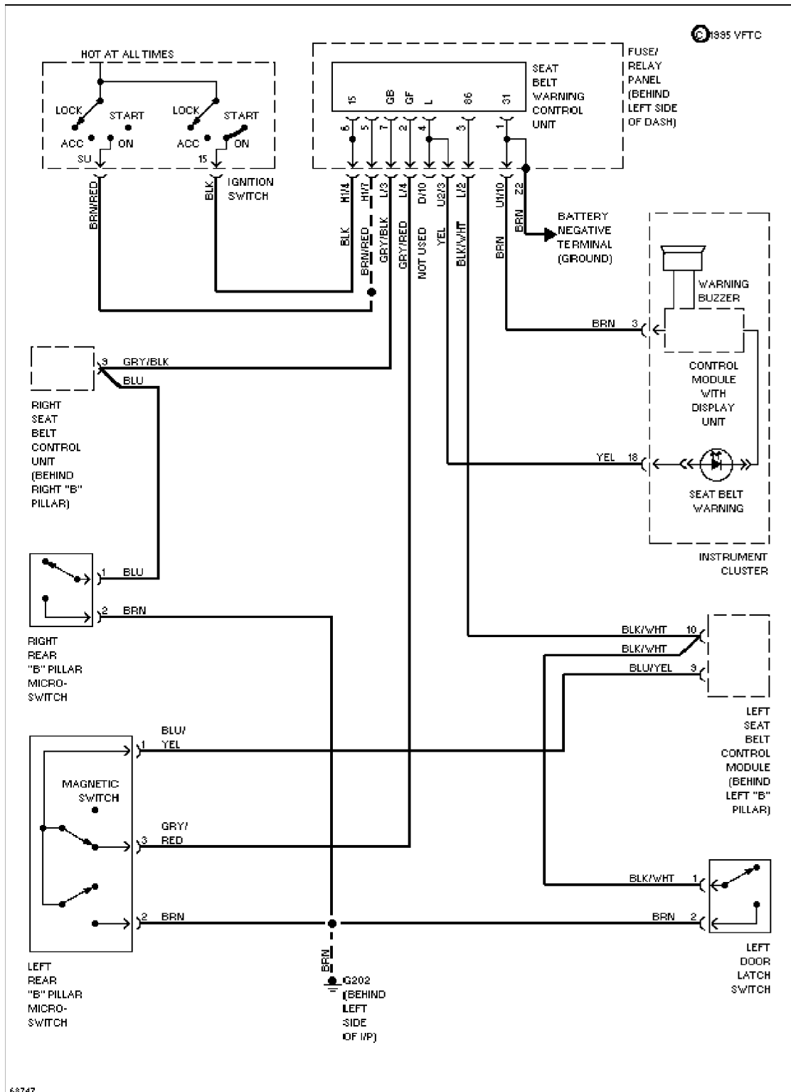
Warning System Circuits, W/ Automatic Seatbelts
