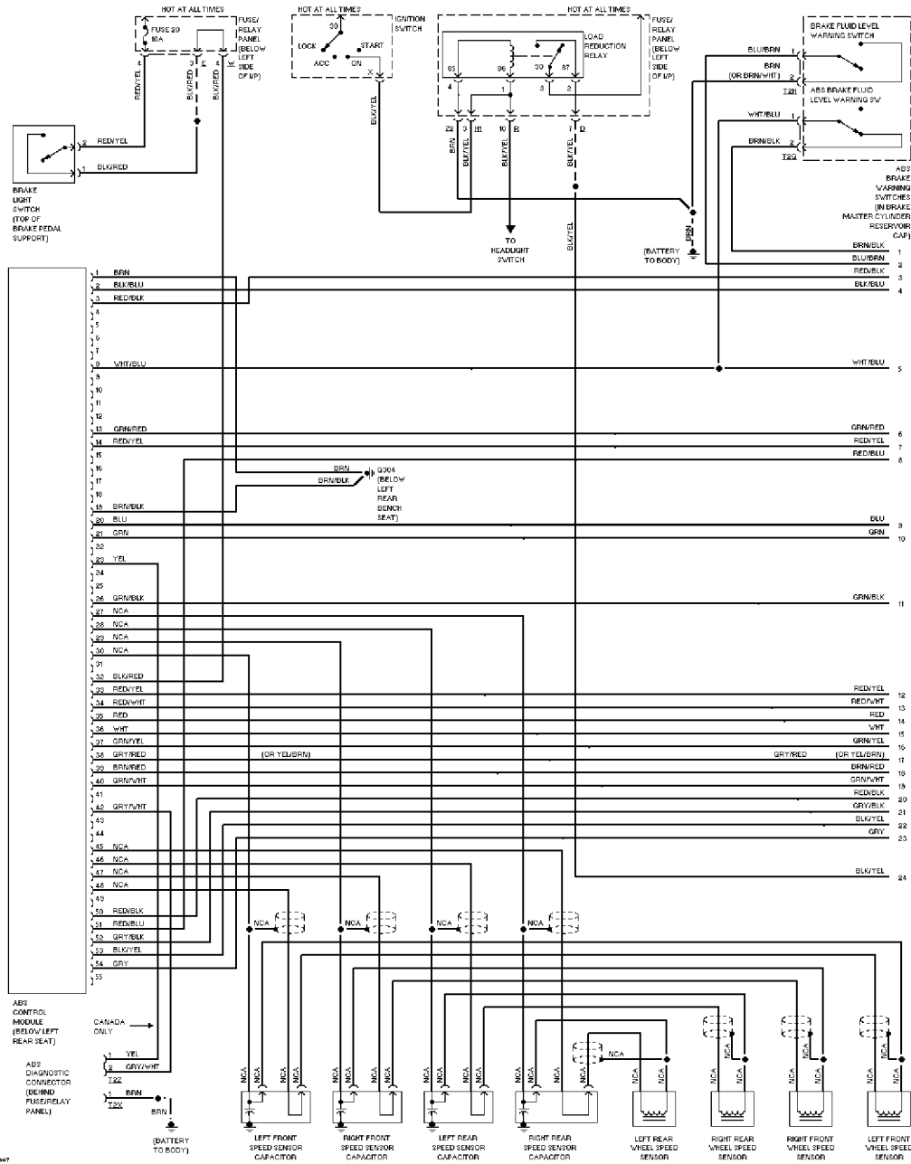
Anti-lock Brake Circuits (1 of 2)
