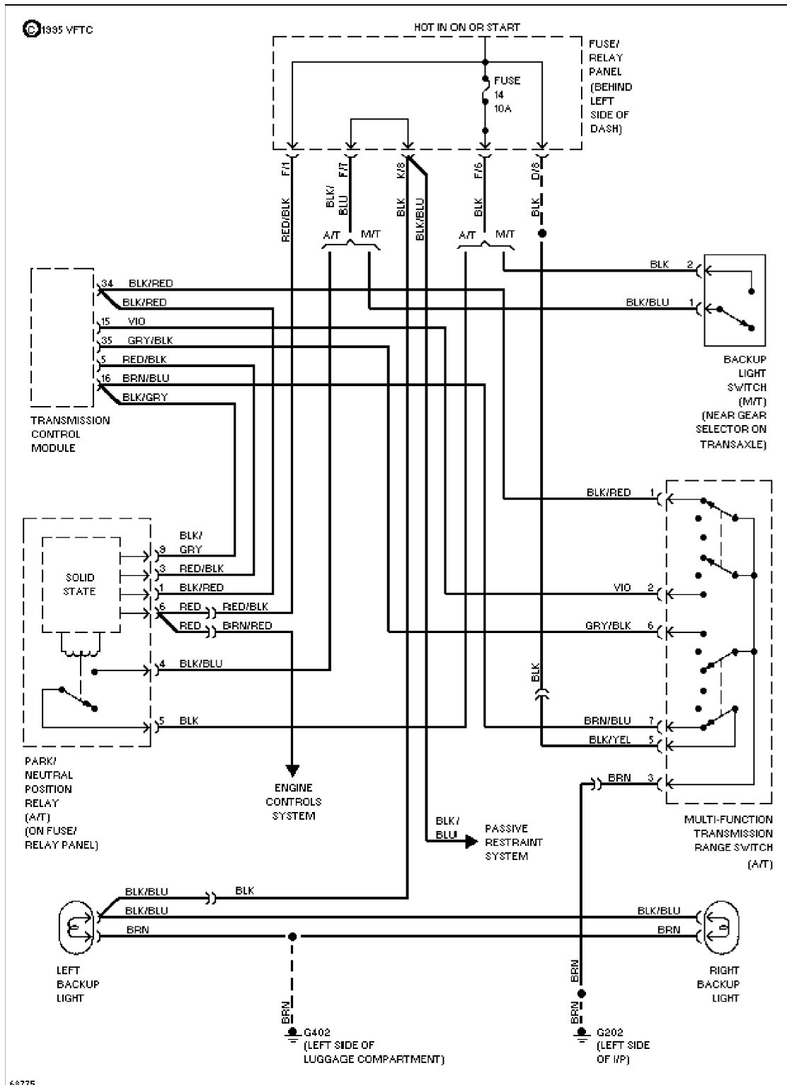
68775 Backup Lamps Circuit
