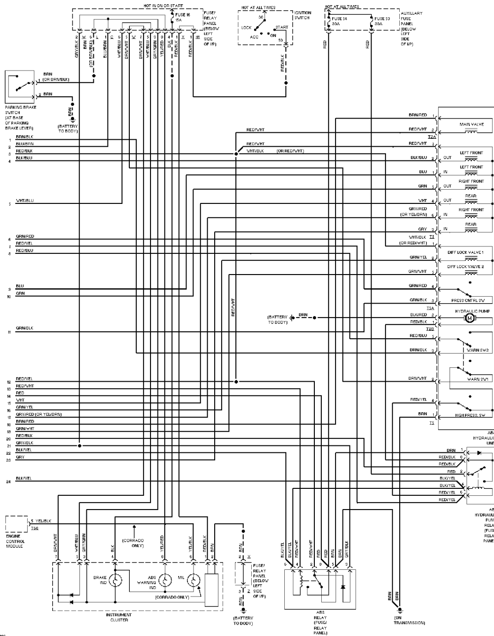
Anti-lock Brake Circuits (2 of 2)
