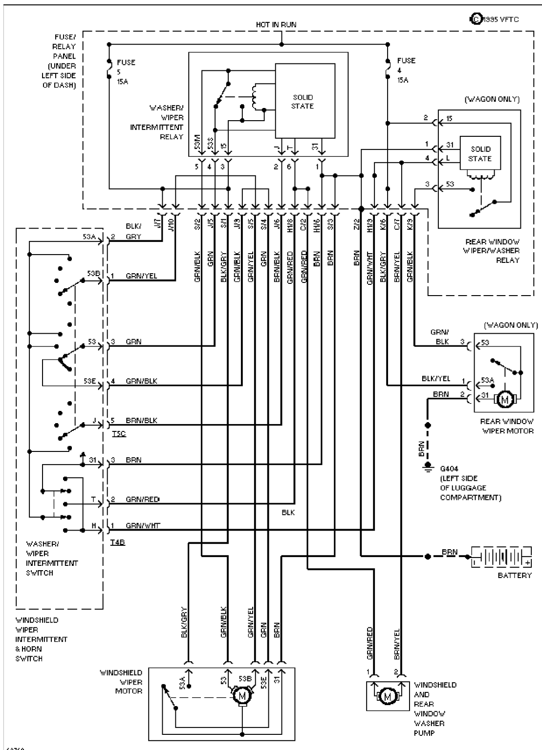
Wiper/Washer Circuit
