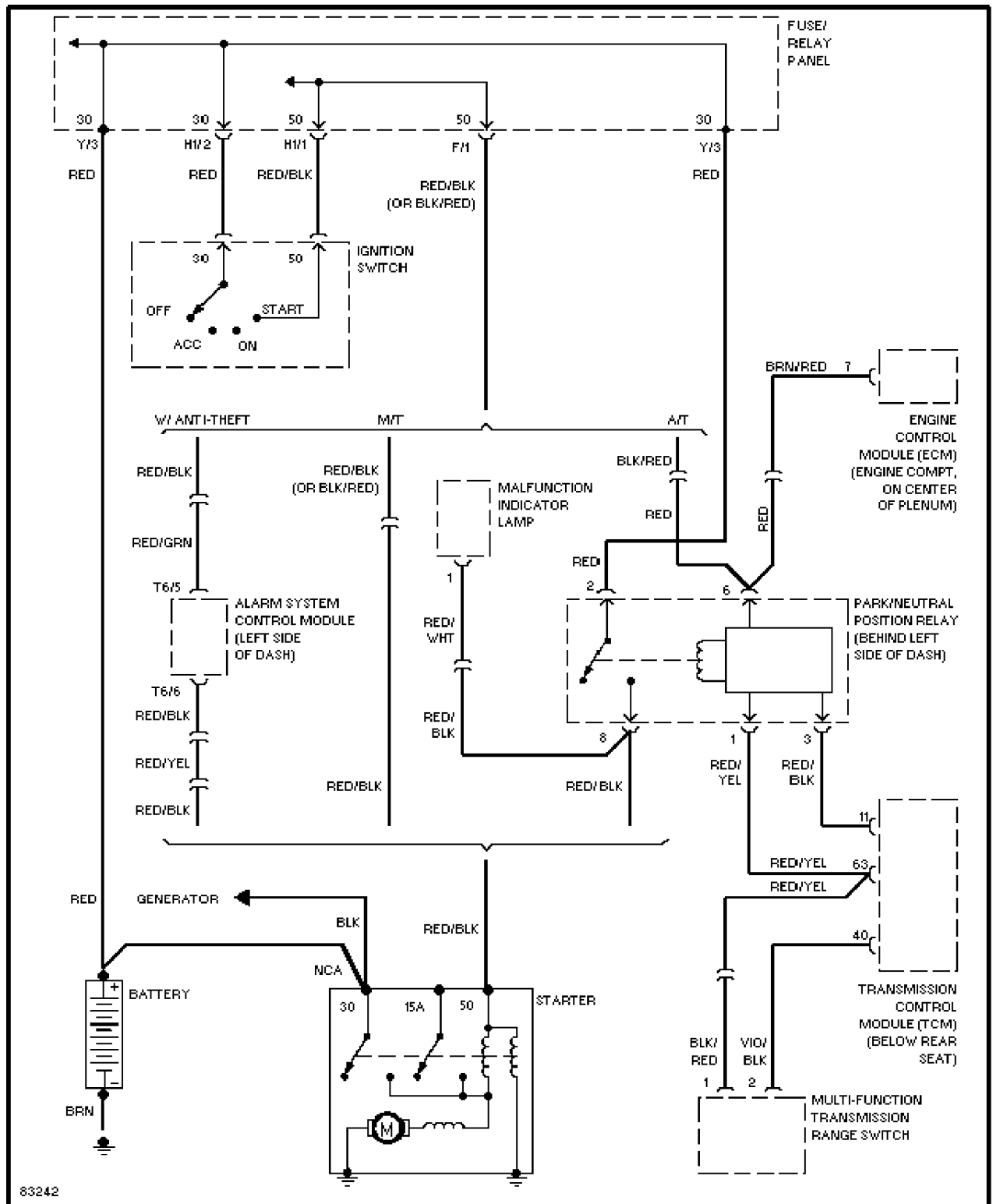
Starting Circuit
