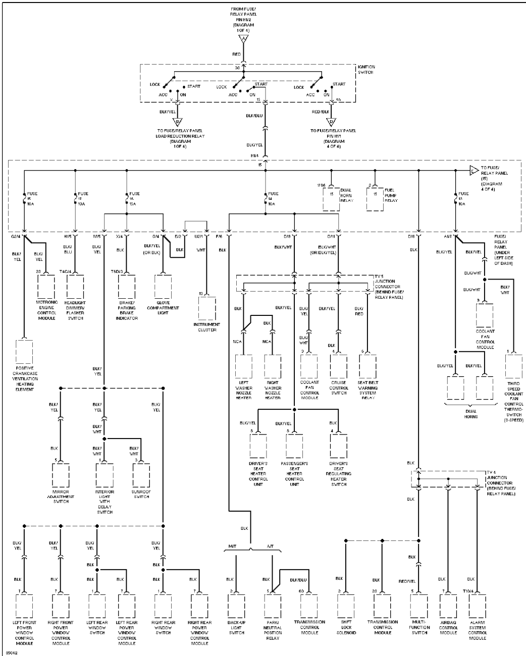
Power Distribution Circuit (2 of 4)
