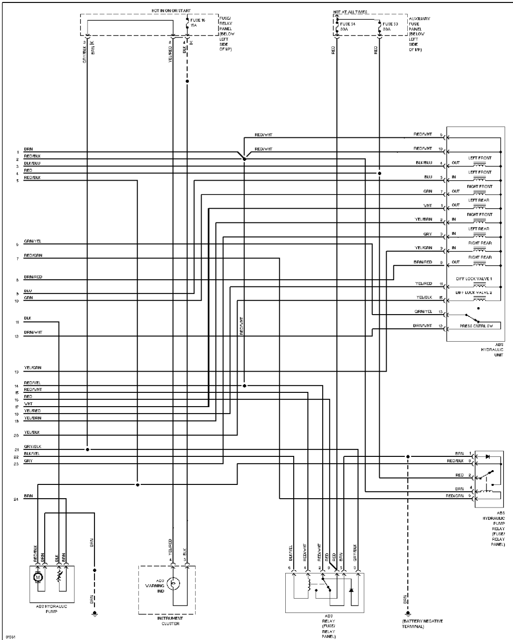
Anti-lock Brake Circuits (2 of 2)
